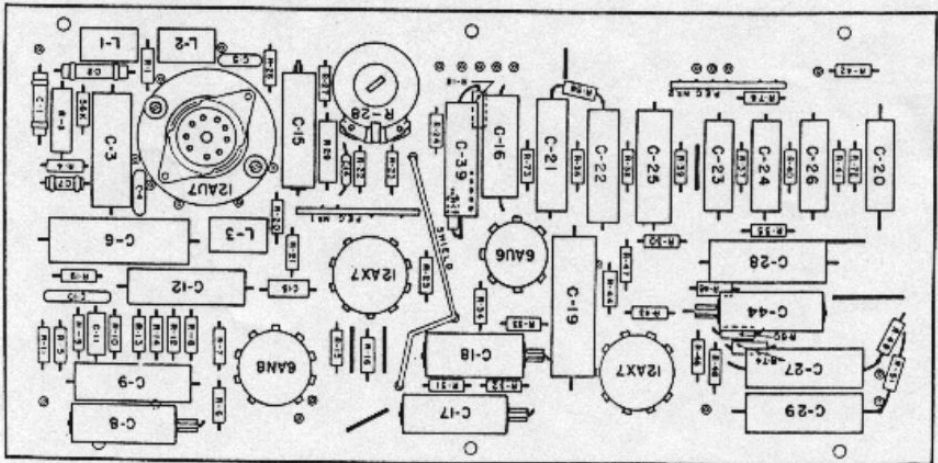
FIG. 104. PRINTED CIRCUIT BOARD (TOP SIDE)
